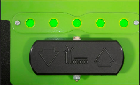
fig. 3B – Front Deck Motor Indicator Lights displaying green under normal operating conditions.
