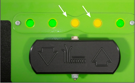
fig. 3C – Front Deck Motor Indicator Lights displaying yellow for blade 3 and 4 indicating tougher mowing conditions for those blades.
