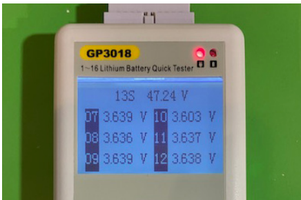
fig. 1F – Next page of cell values.
