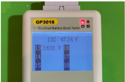
fig. 1G – Last page of cell values.
