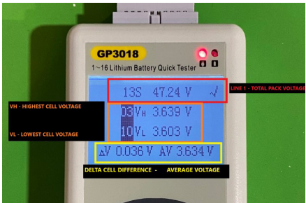
fig. 1D – Main page values.
